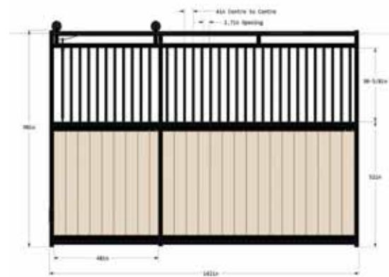
VERTICAL RAIL DIVIDER
